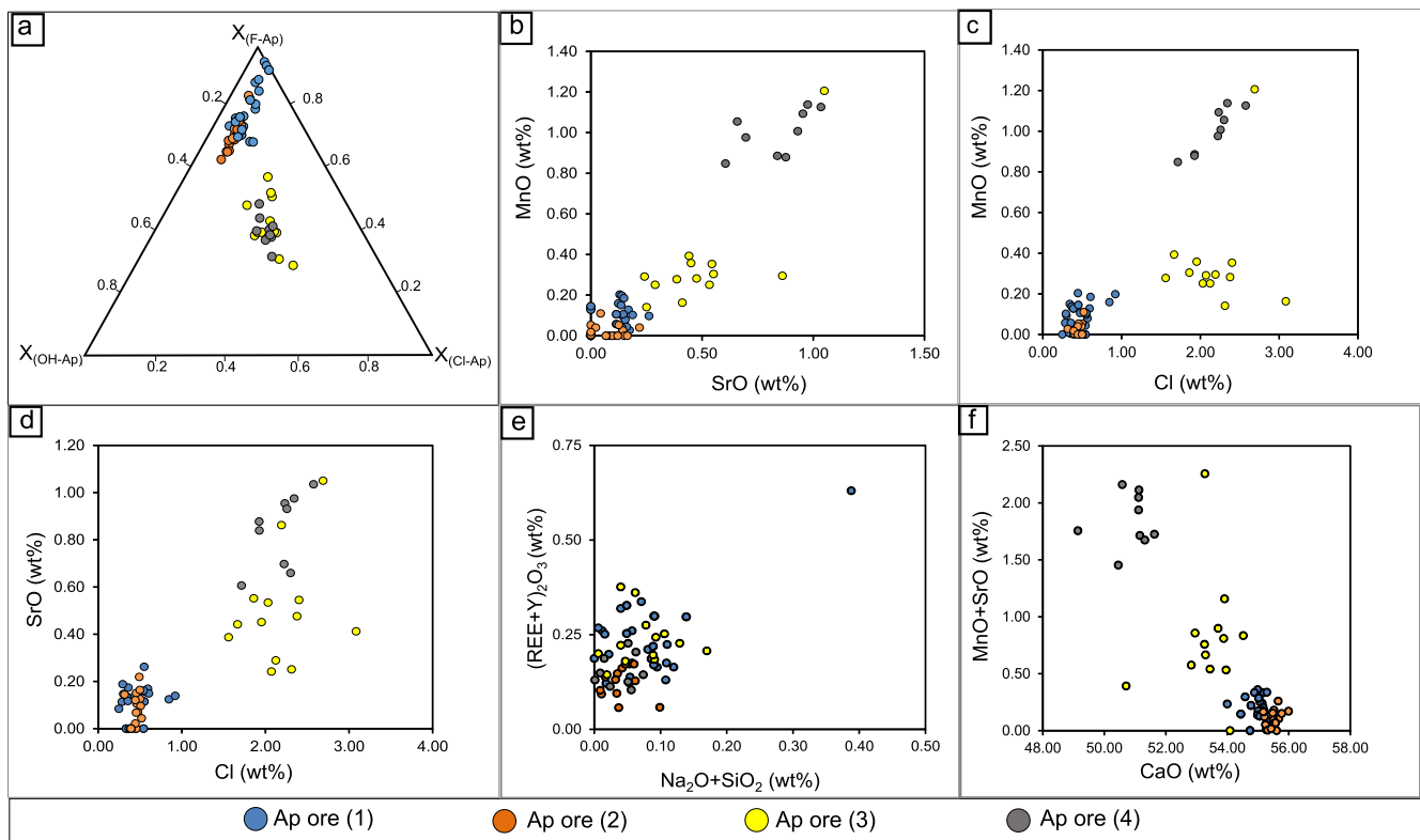
Fig. 5. a) Ternary X_{FAP} - X_{ClAP} - X_{OHAP} diagram showing substitution relations on the halogen site for the PKF apatites from all four ore types. b) Plot of SrO vs. MnO (wt %) for apatite from the PKF IOA ores. c) MnO vs. Cl (wt %) plot for apatite from the PKF IOA ores. d) SrO vs. Cl (wt %) for apatite from the PKF IOA ores. e) Na_2O + SiO_2 vs. (Y + REE)_2O_3 for the apatite from the PKF apatite ore bodies, showing a uniform very low REE content in the apatite from all four ore types. f) Negative correlation of CaO vs. MnO + SrO (wt %) in apatite.
