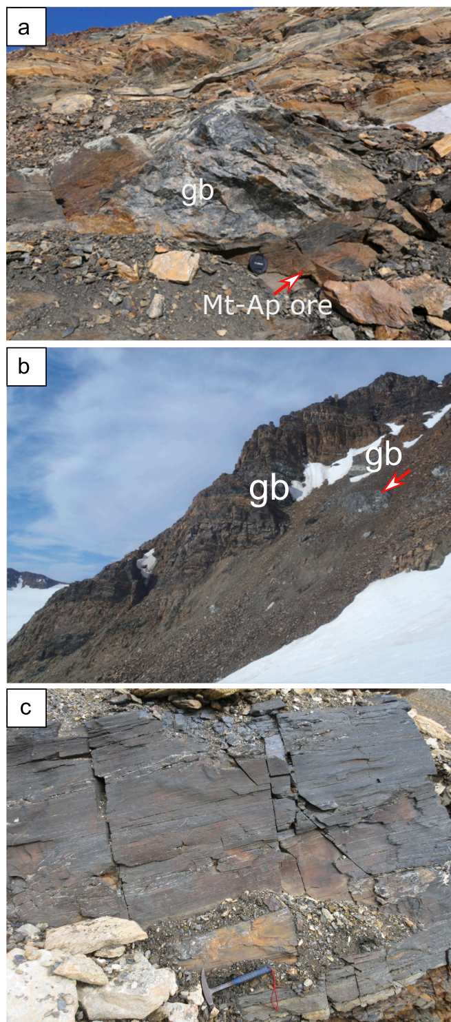
Fig. 2. Field photographs of the PKF IOA ore bodies. a) Lenticular meta-gabbro body (gb) within metasediments of the Craigtoppane Unit in sharp tectonic contact with a Type (1) ore body (south slope of Laurantzonfjellet). b) Lenticular-shape boudin of Type (3) ore in spatial association with meta-ferrogabbros (gb) within cataclased calcareous and silicious metasediments (south pillar of Boureéffjellet). The red arrow points to IOA ore bodies. c) Outcrop of banded Type (2) ore emplaced in slaty silicious metasediments. Note the pronounced slaty cleavage of the ore body. Mineral abbreviations: Mt – magnetite, Ap – apatite.
