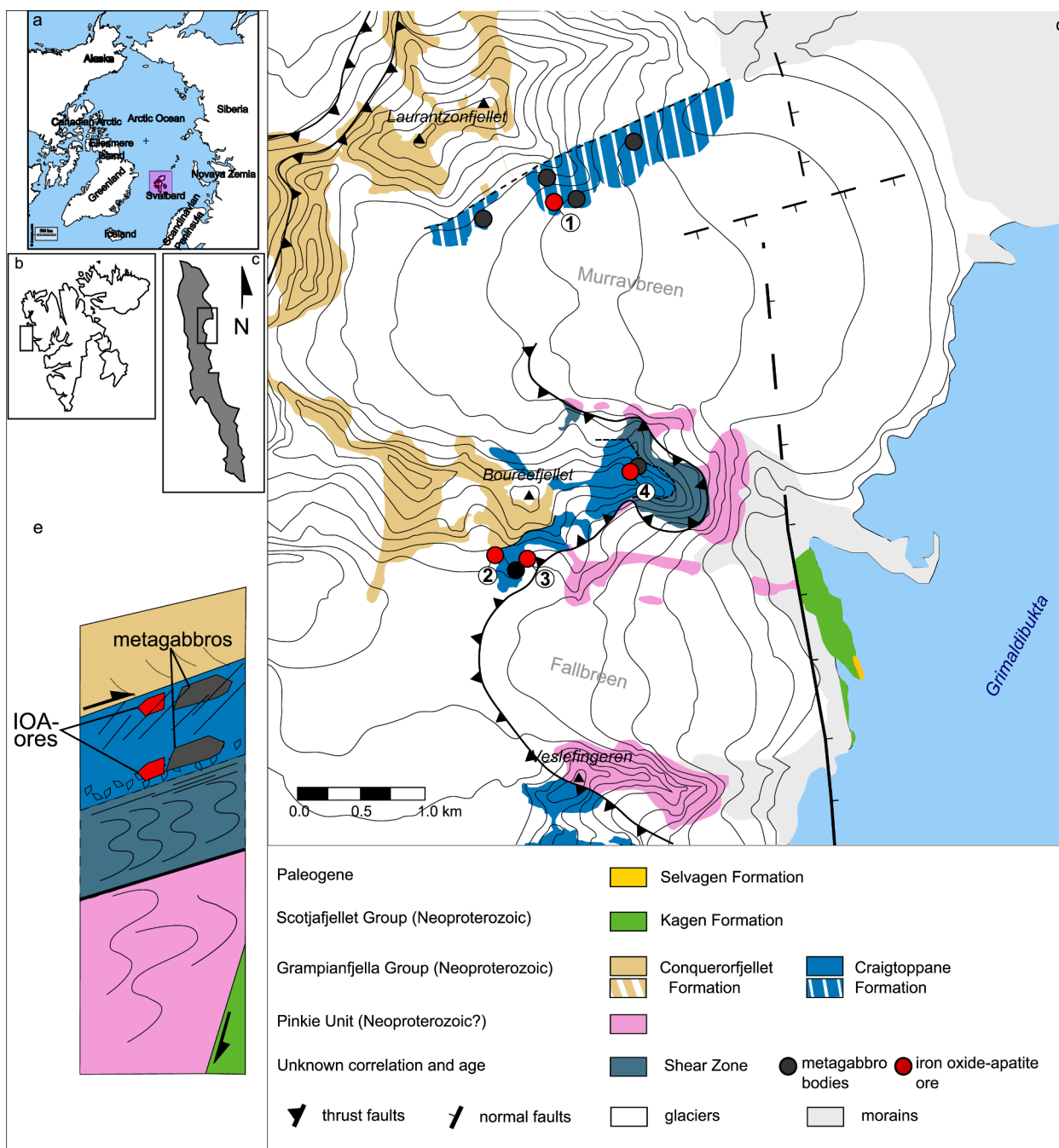
Fig. 1. a) Location of Svalbard Archipelago. b) Location of Prins Karls Forland in the Svalbard Archipelago. c) Investigated area on Prins Karls Forland. d) Simplified geological map of the research area (adapted from Hjelle et al. 1999; Schneider et al. 2019; Dallmann 2020). The ore body numbers refer to the textural types distinguished in Table 1. Diagonal stripes indicate inferred tectonostratigraphic affiliation. e) Schematic profile across the BSZ and Pinkie Unit (modified after Schneider et al. 2019).
